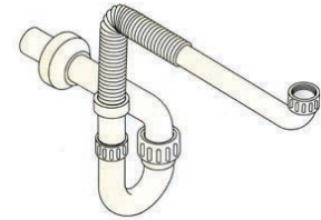
Space Saver Bottle Trap Designed to Maximise Vanity Unit Draw Space Can be Cut to Suit 1 1/4" White Code: BDP-TRP-120-WH
